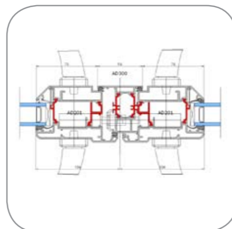
Interlock Detail
