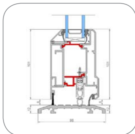
Cill Detail
